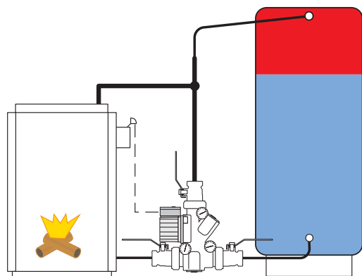
Laddomat 21-100
